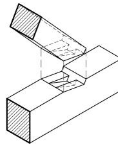
12. 흘림장부안장맞춤
